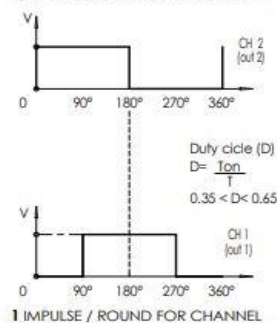
OUTPUT SIGNAL OF HALL SENSOR
